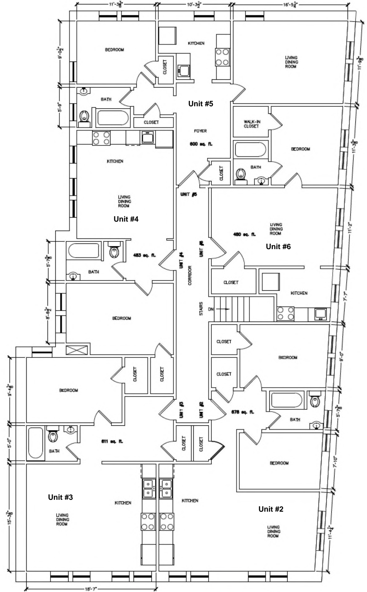
SECOND FLOOR - PROPOSED
