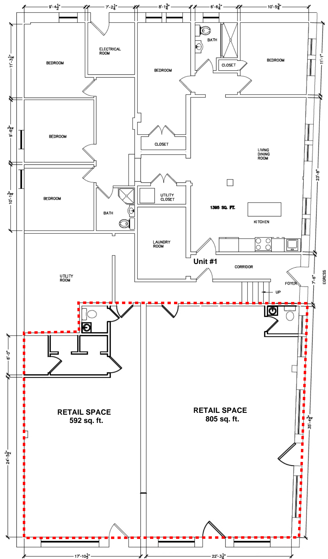
FIRST FLOOR - EXISTING
